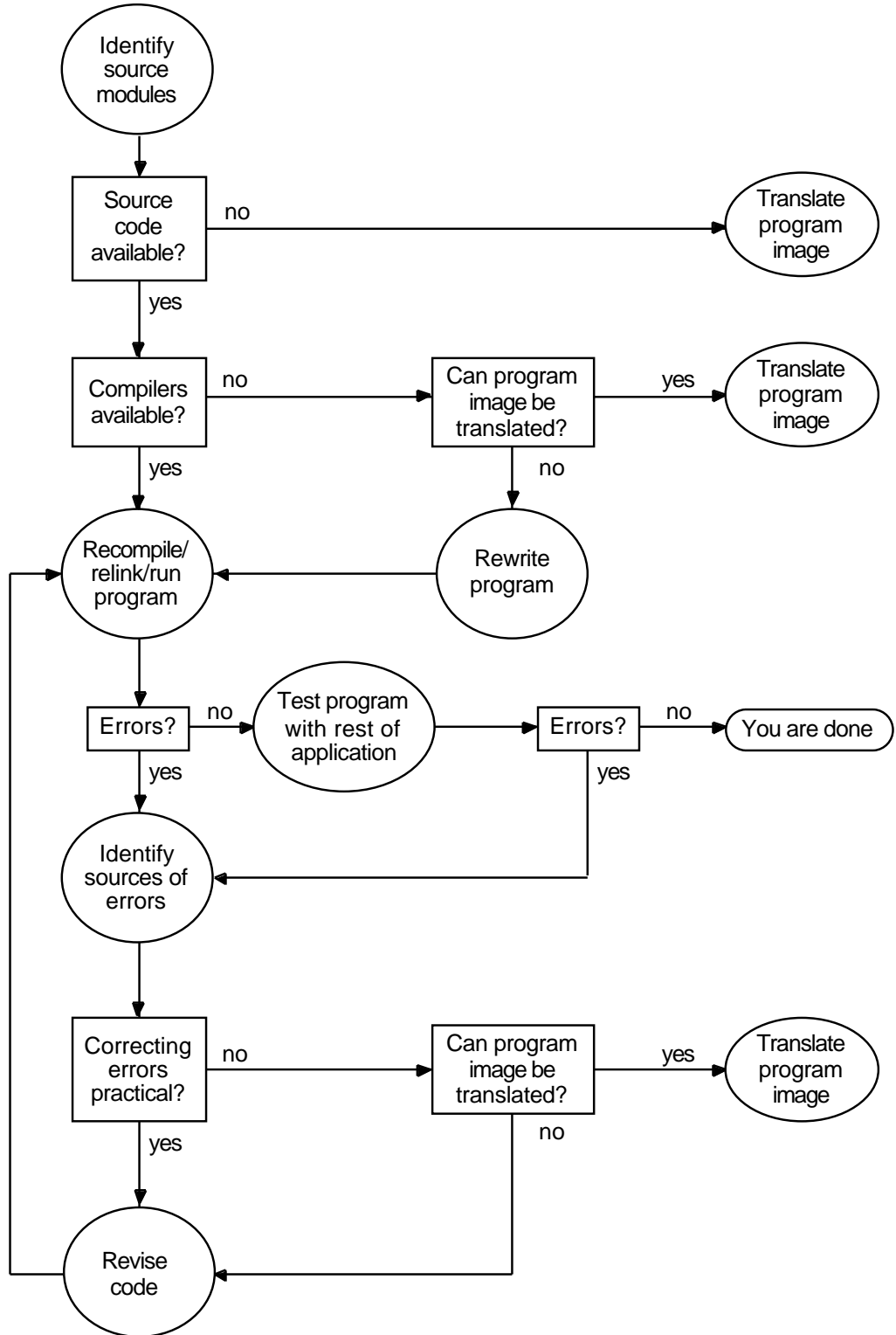
Figure 4-1 Migrating a Program
