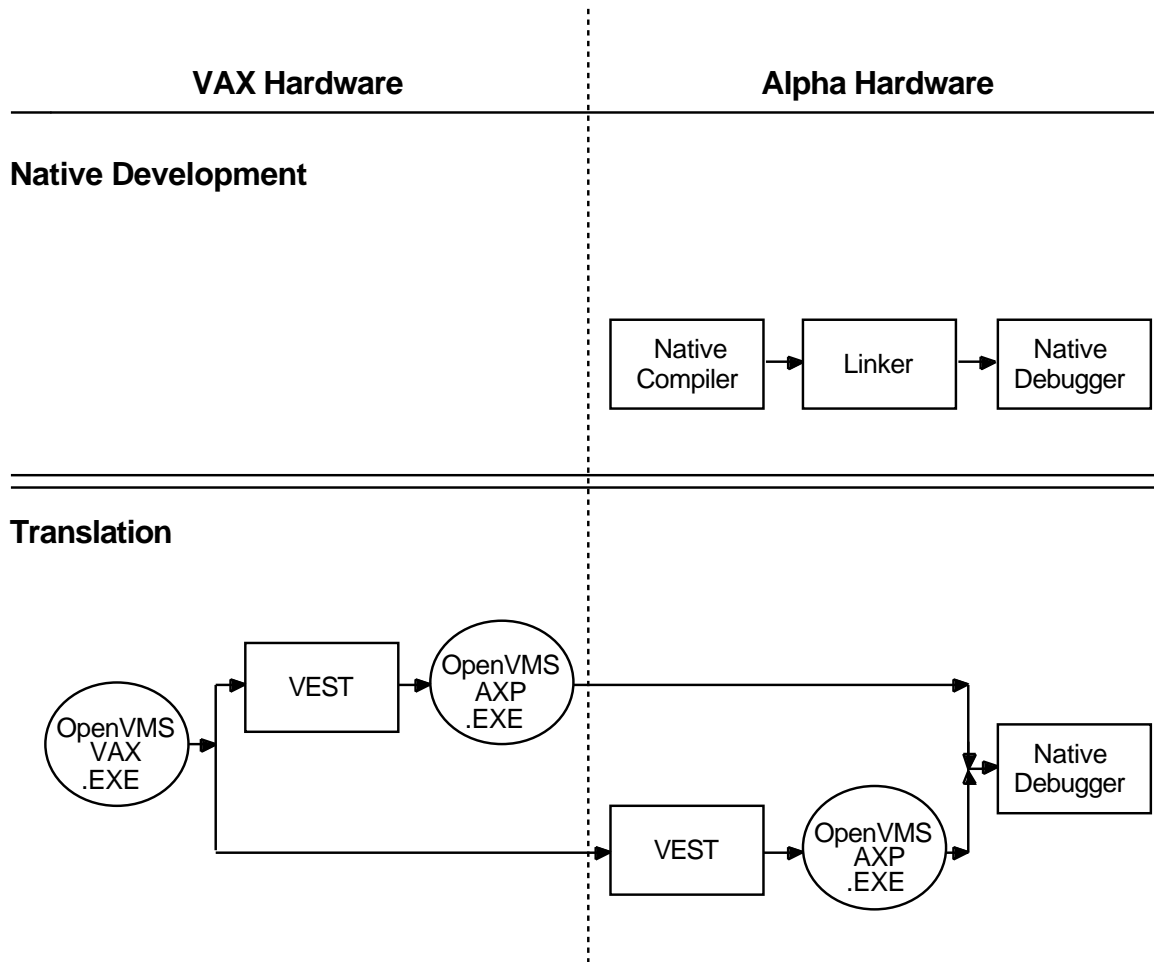
Figure 6-1 Migration Environments and Tools
