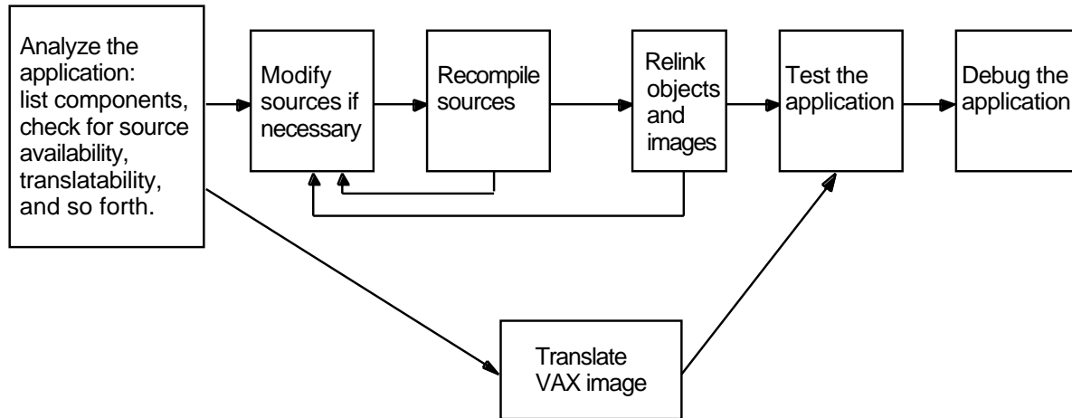
Figure 2-1 Methods for Moving VAX Applications to an AXP System
